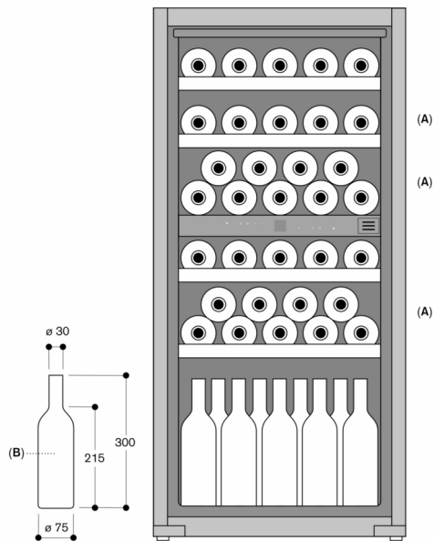
A: Suitable area for storage of magnum bottles in standard tray configuration B: 0.75 litres Measurements in mm
