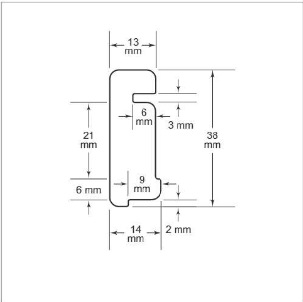
Wood facing profile—Designer Series and Model ICBCL3050W
