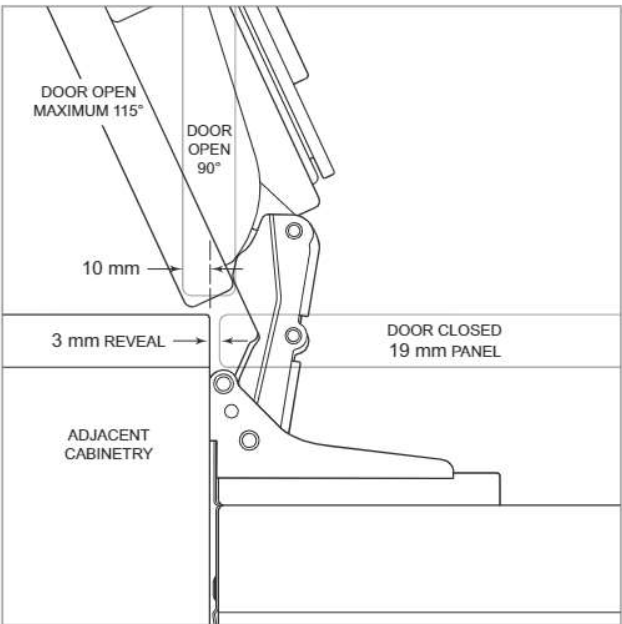
Maximum door opening (top view)
