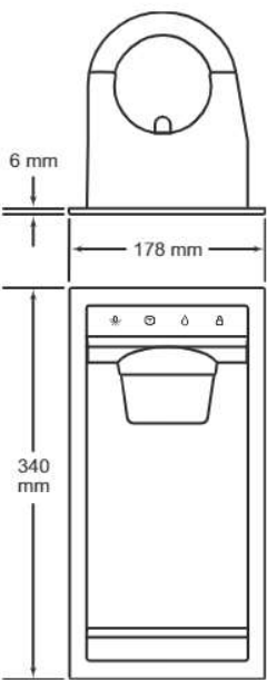
Dispenser dimensions
