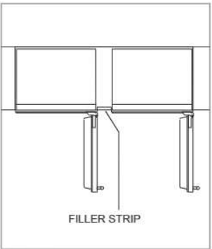
Same side hinges
