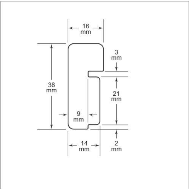
Wood facing profile—Model ICBDEU2450W
