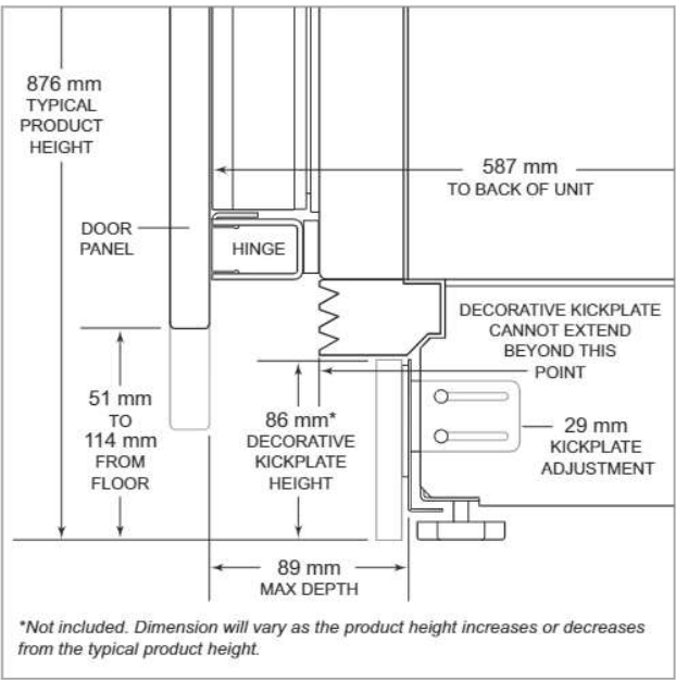
Toe kick clearance (side view)
