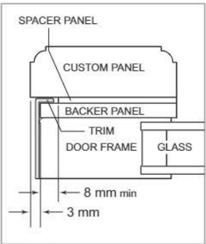
Panel assembly cross section (overlay)
