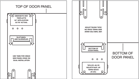
Door panel template—top. Door panel template—bottom (tall model).
