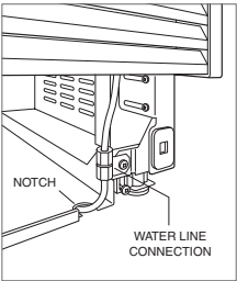
Water line (ICBIW-30CI).
