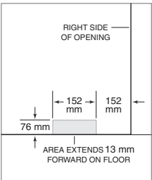
Water supply location (ICBIW-30CI).
