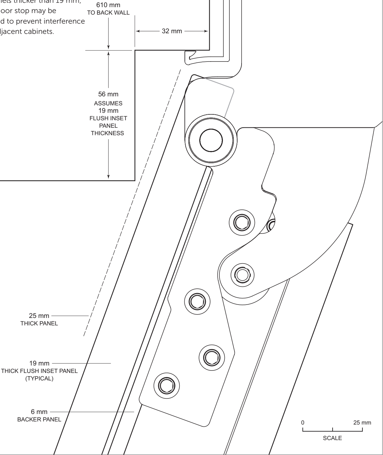
110° door opening (top view)
